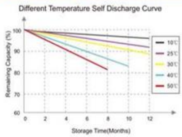
Self Discharge Characteristics Curve
