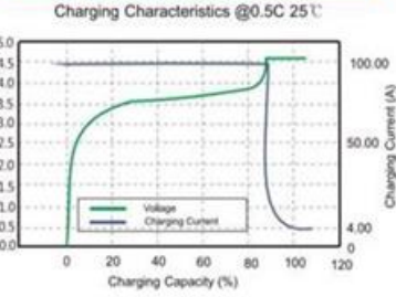
Charging Characteristics
