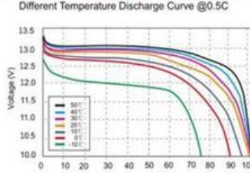
Different Temperature Discharge Curve
