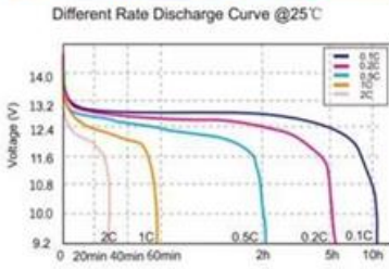
Different Rate Discharge Curve
