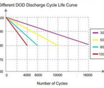
Cycle Life Curve
